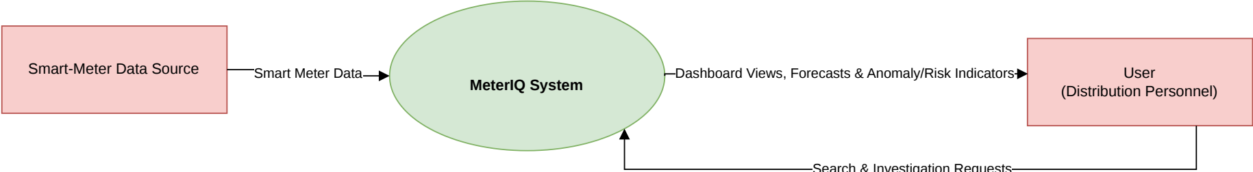
MeterIQ: Data FLOW Diagram Level-0
