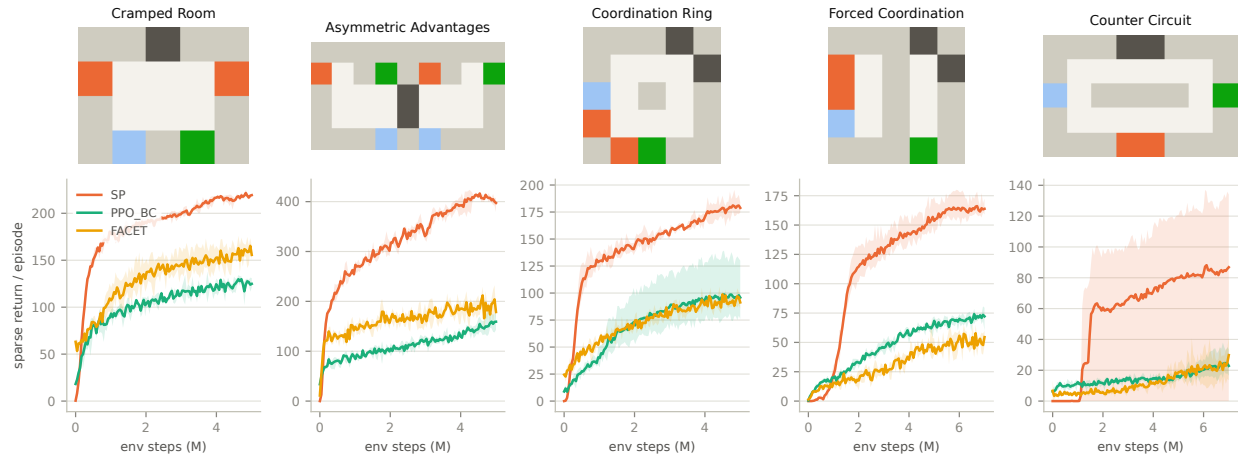
Figure 1: Top: the five layouts (orange = onion dispensers, blue = dish dispensers, dark = pots, green = serving windows). Bottom: training curves (sparse return per episode; mean over 3 seeds, min-max band). Curves are measured against each method’s training partners and are not comparable across methods—SP plays with a copy of itself, PPO BC with a stochastic human model, FACET with its mixed pool. One SP seed on Counter Circuit never scored (flat 0 for 7M steps), a known failure mode of self-play on this layout.
