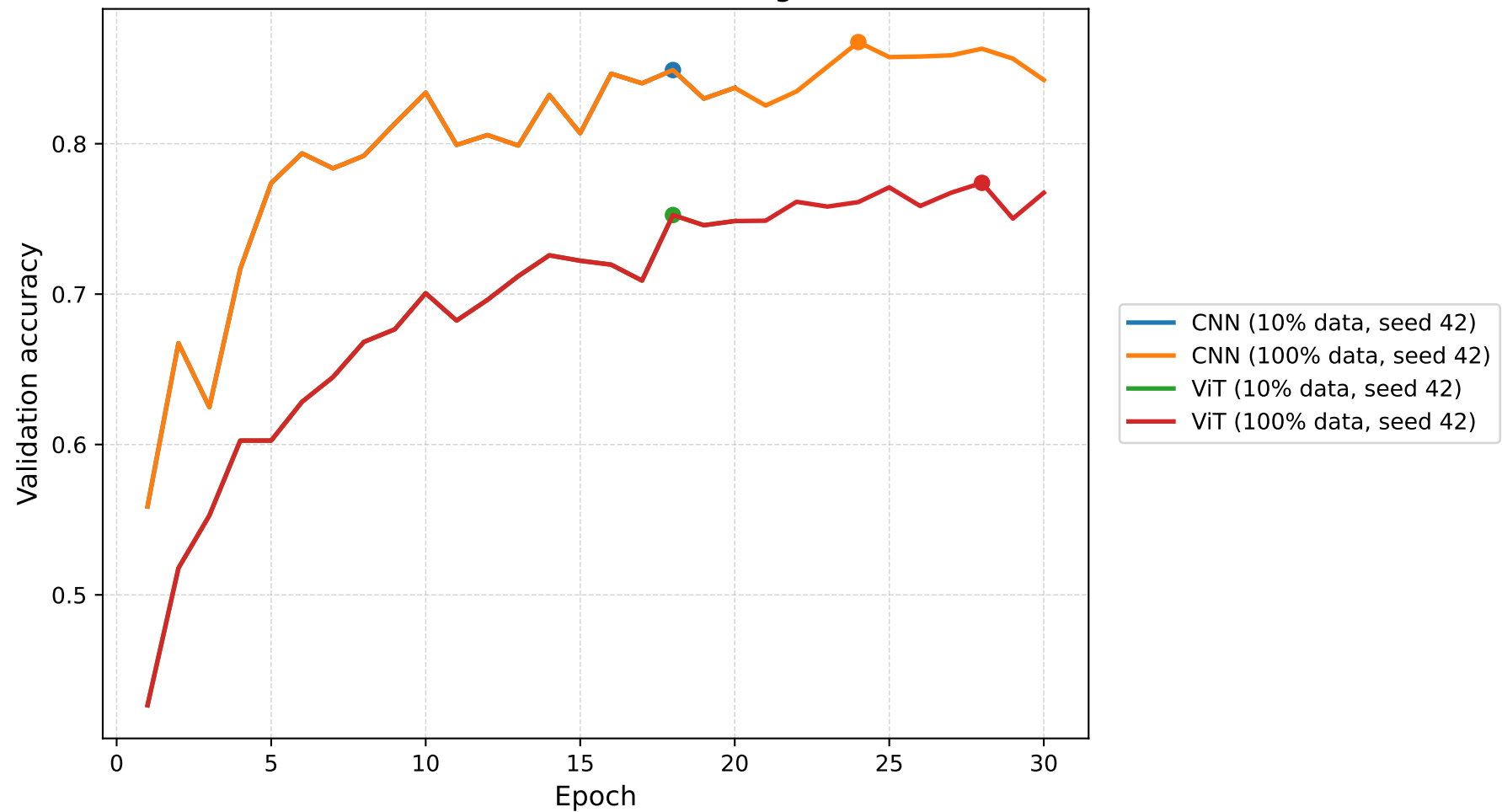
CNN vs ViT on CIFAR-10 (learning curves)
