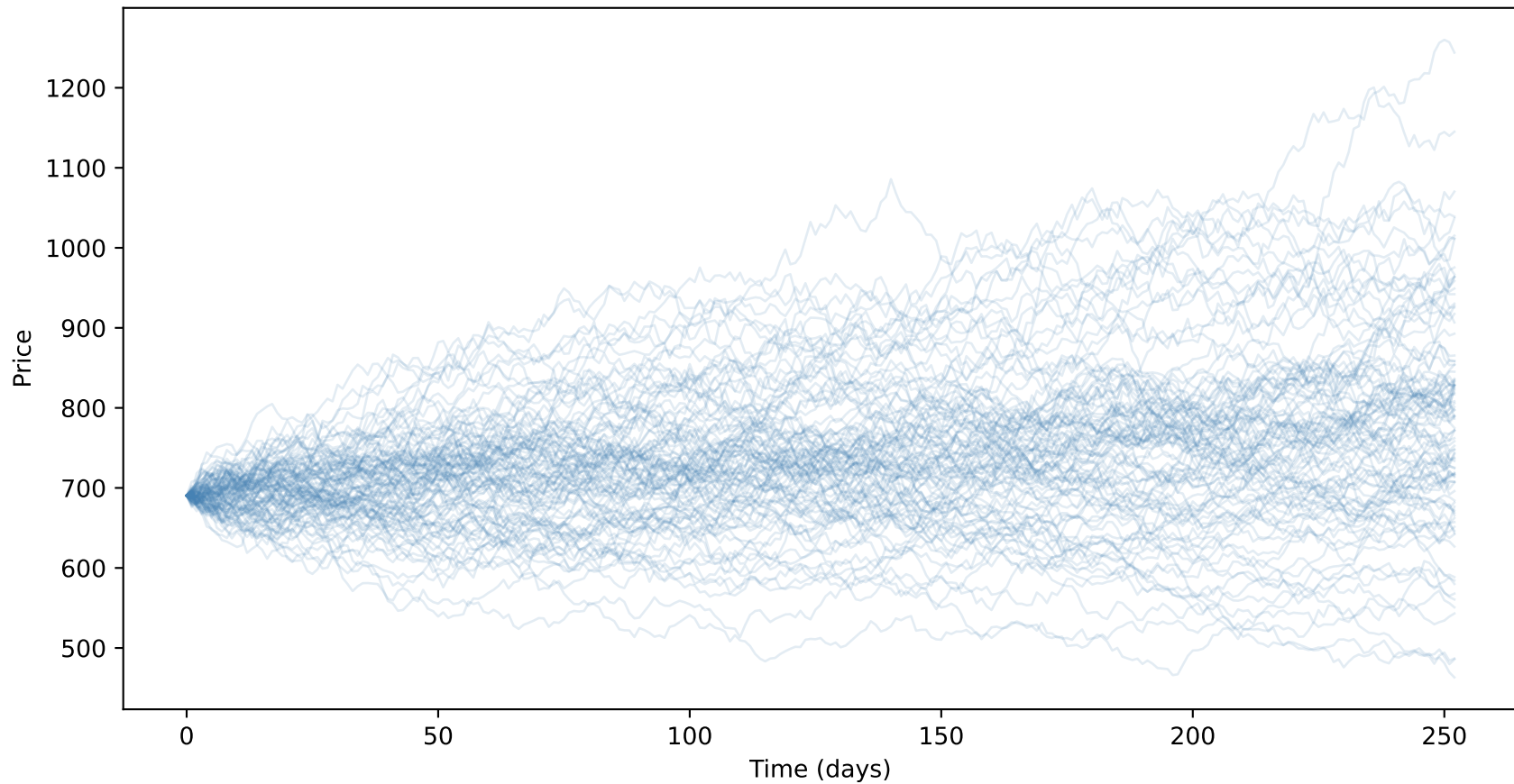
Monte Carlo Price Paths (Fan Chart)
