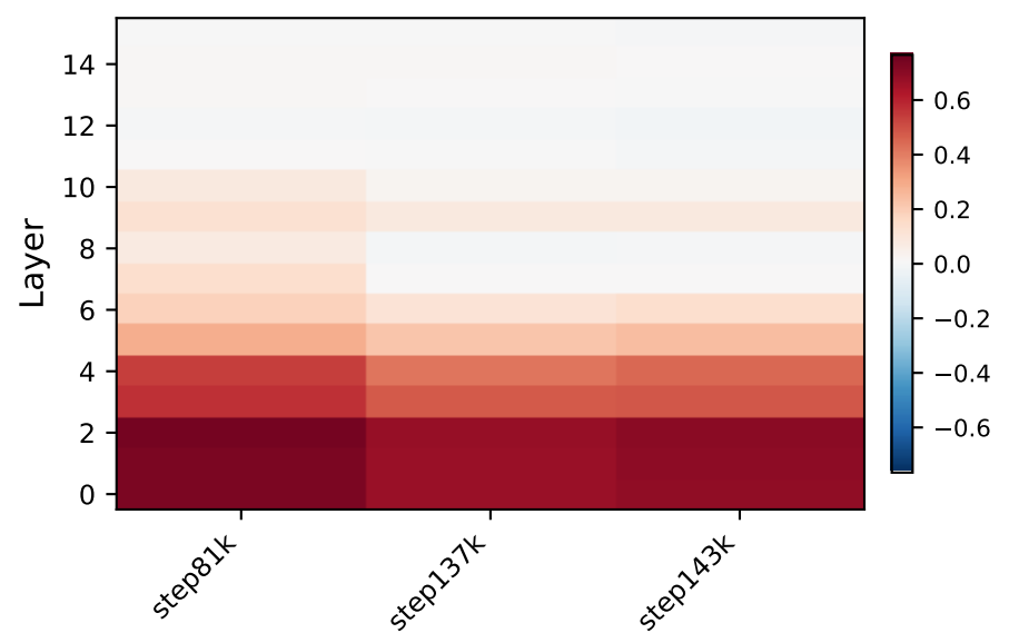
Effect of MLP window restore
