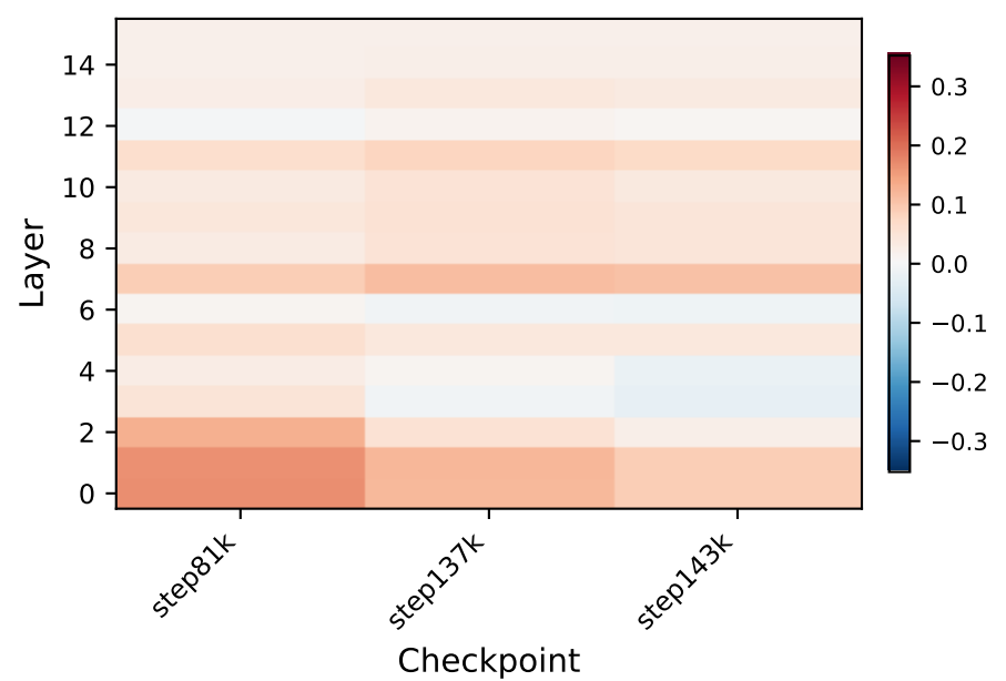
Effect of Attn window restore
