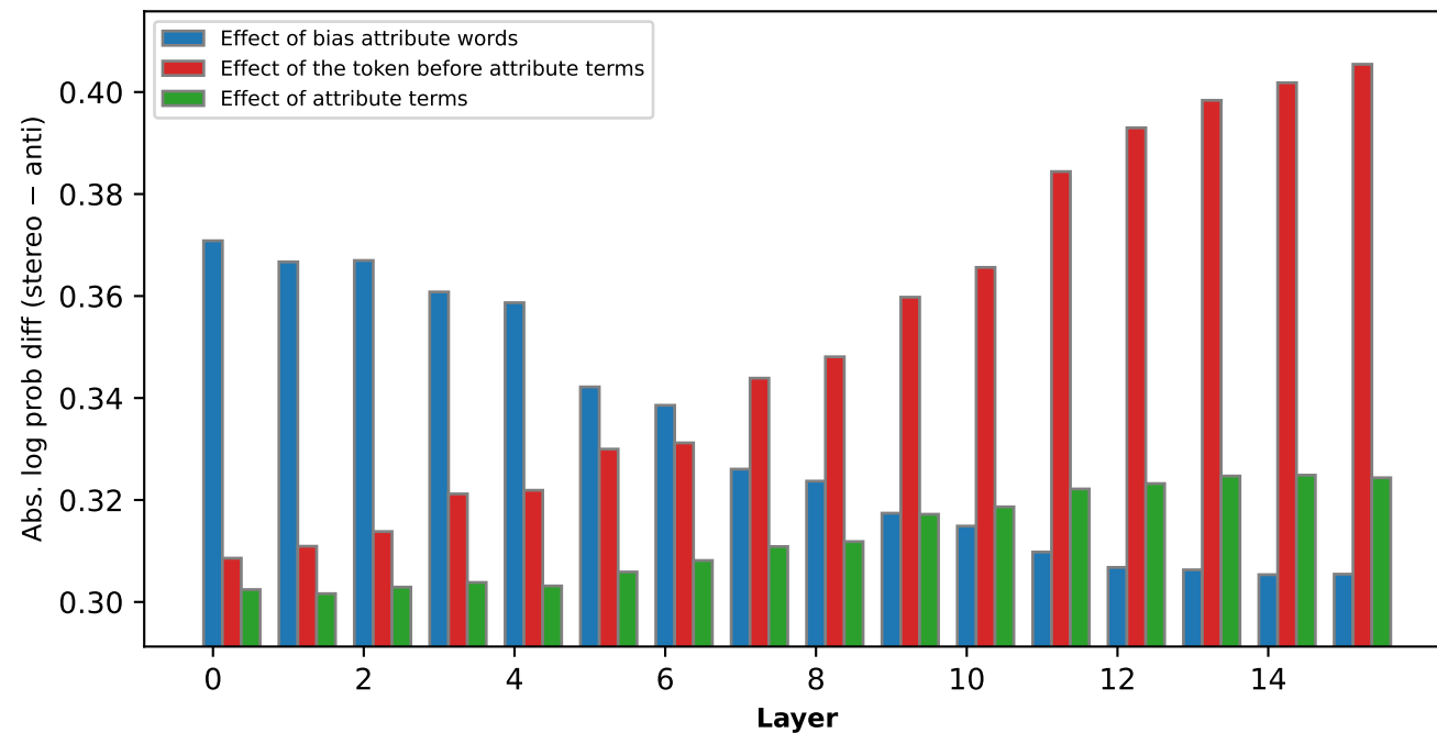
step2000
