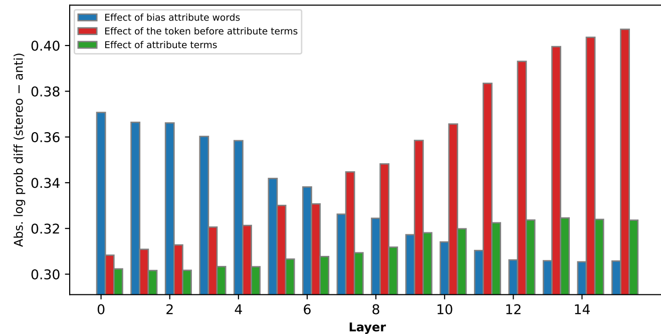
step2600
