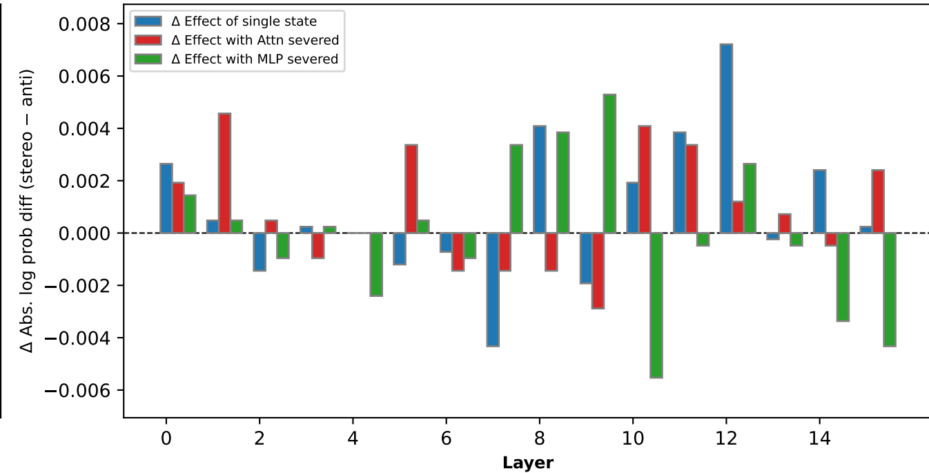
OLMo-2-0425-1B-Instruct — Religion bias: \Delta per layer vs. previous checkpoint Bars show change in abs. log prob diff (curr – prev) at each layer. Positive = more causal effect acquired. Y-axis fixed across all intervals.
