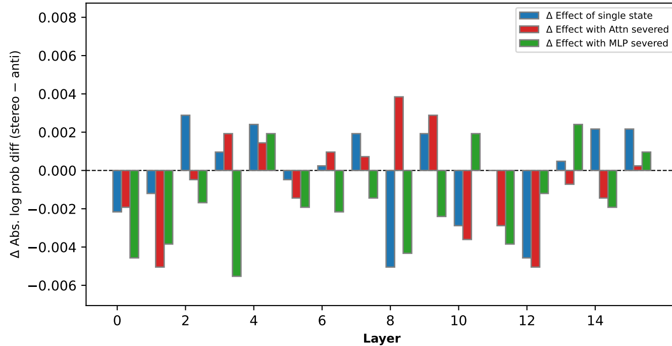
OLMo-2-0425-1B-Instruct — Religion bias: \Delta per layer vs. previous checkpoint Bars show change in abs. log prob diff (curr – prev) at each layer. Positive = more causal effect acquired. Y-axis fixed across all intervals.
