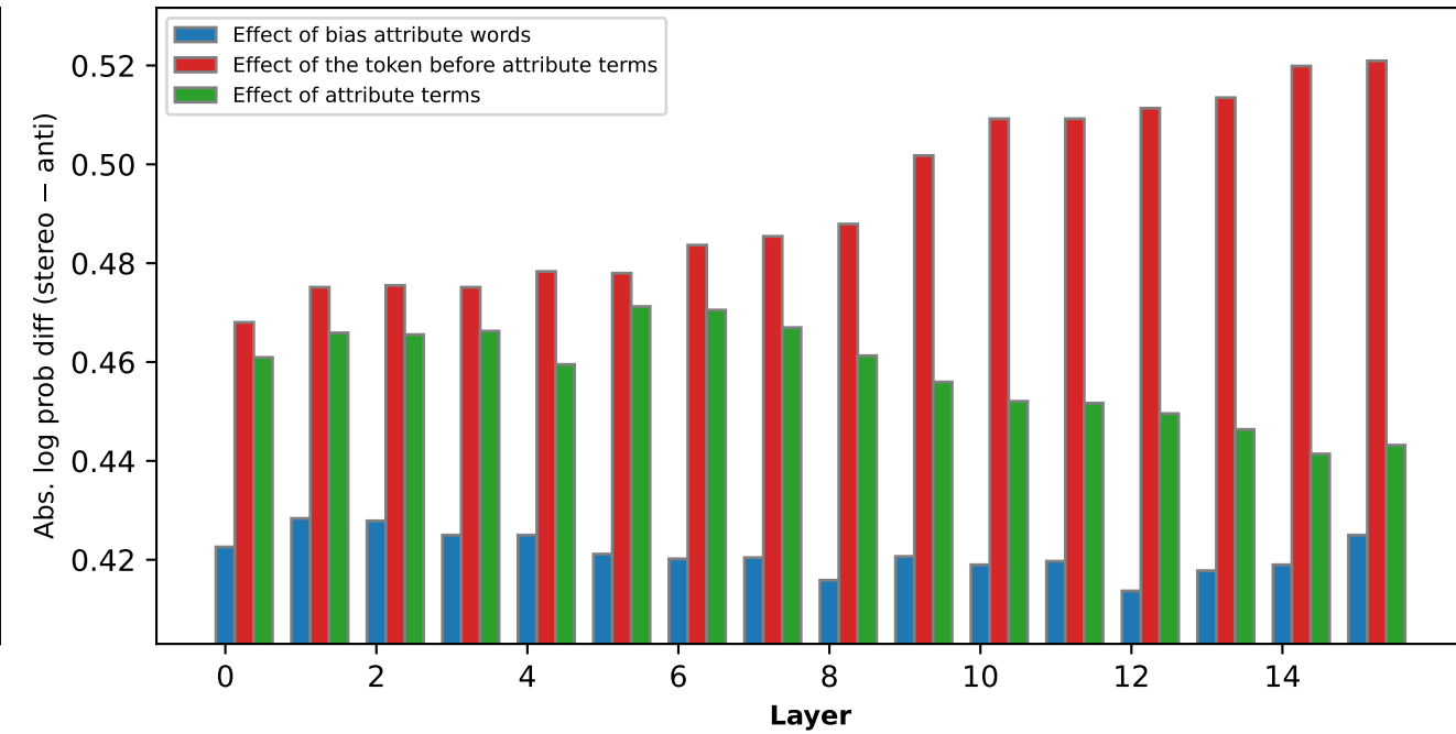
step2600
