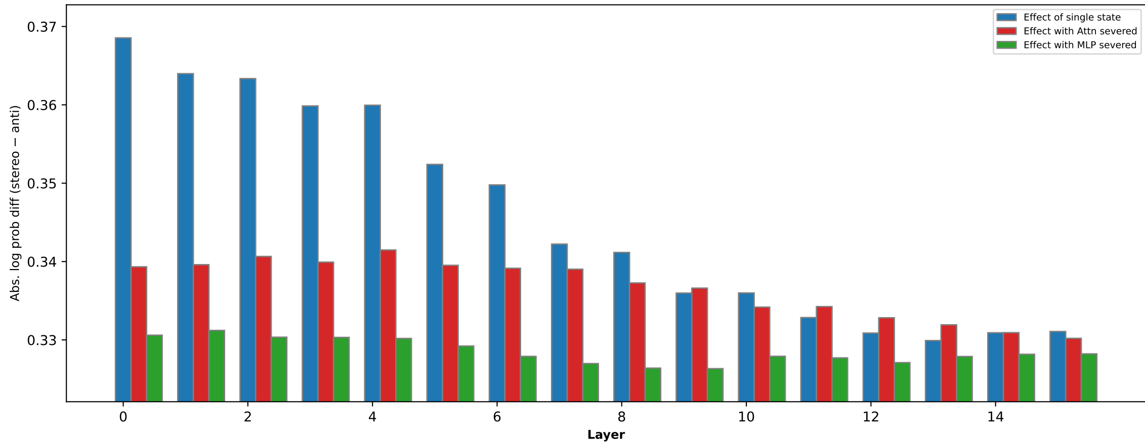
Gender bias effect of states (OLMo-2-0425-1B-Instruct [step2000])
