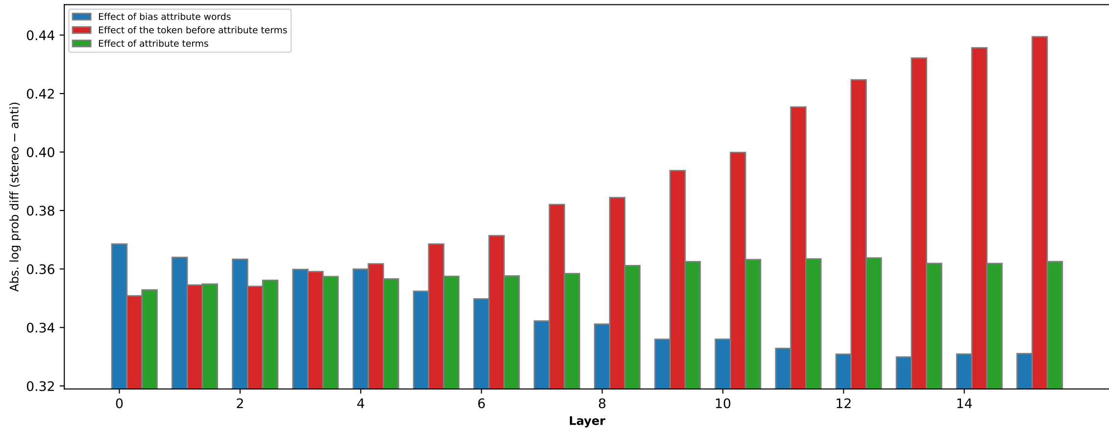
Gender bias effect of different words (OLMo-2-0425-1B-Instruct [step2000])
