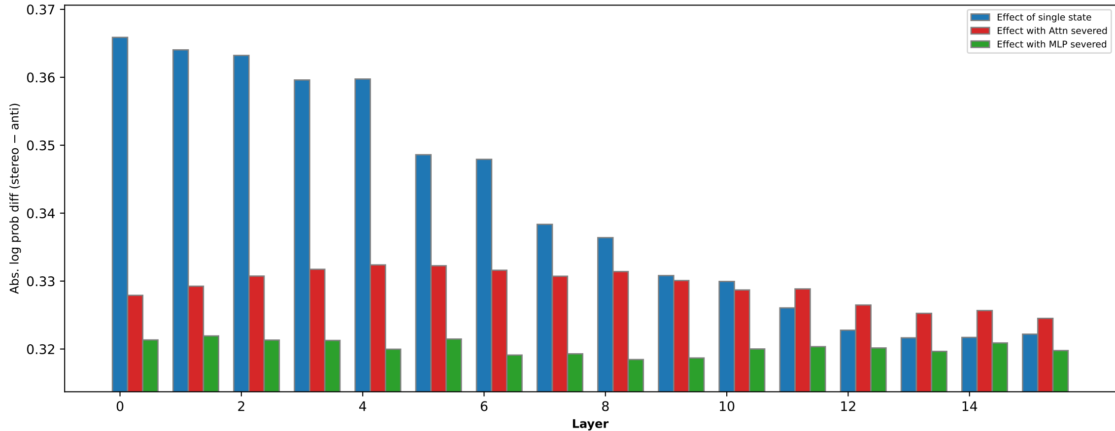
Race bias effect of states (OLMo-2-0425-1B-Instruct [step2600])
