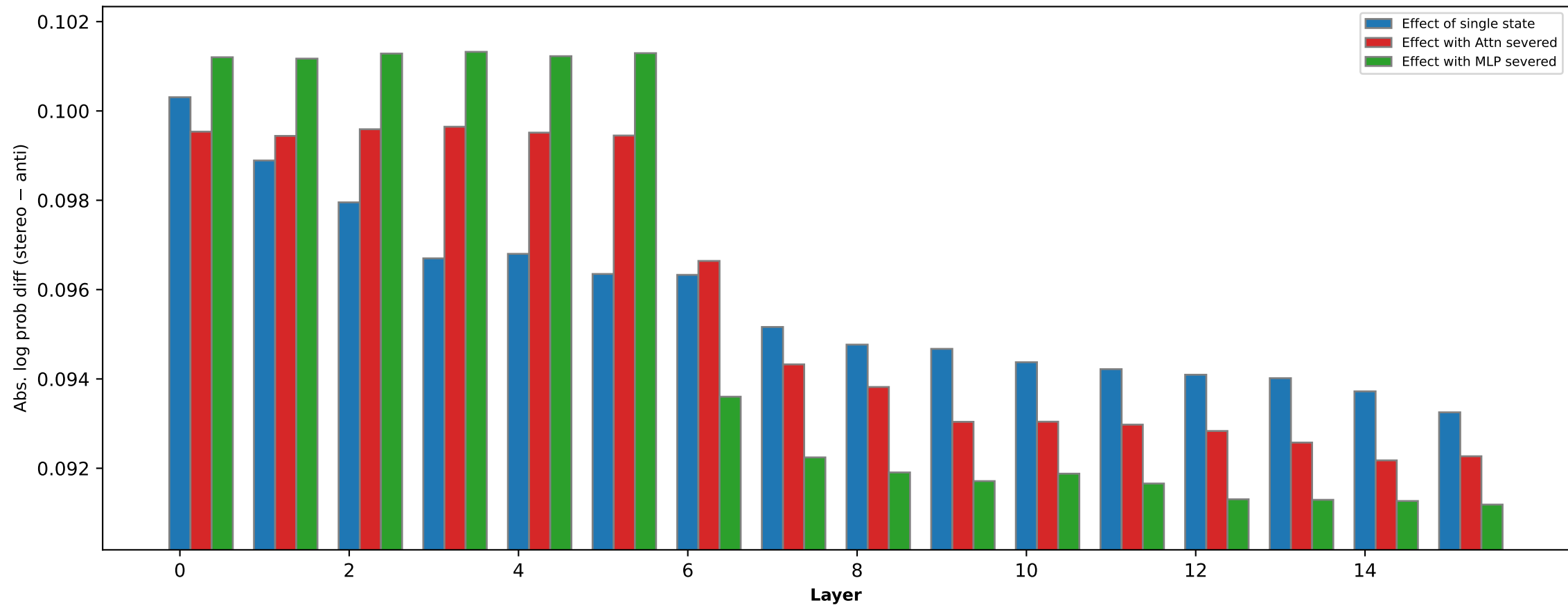
Profession bias effect of states (OLMo-2-0425-1B [0B])
