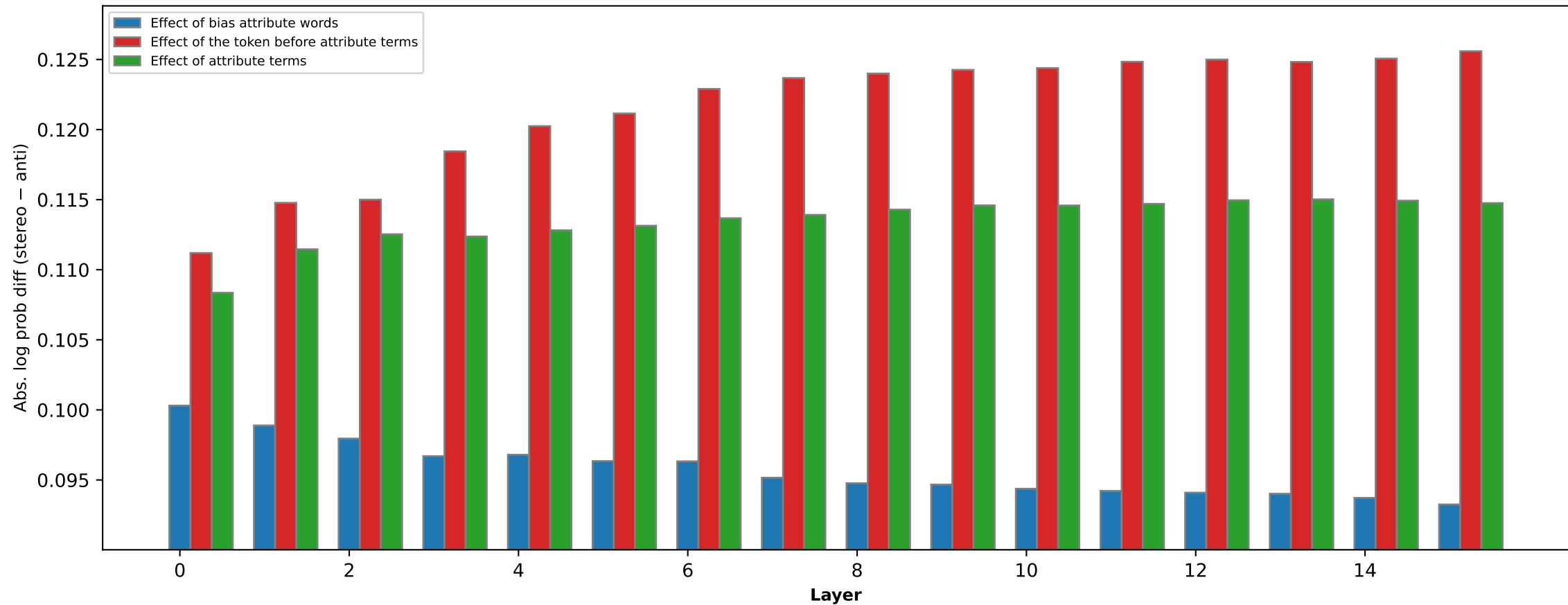
Profession bias effect of different words (OLMo-2-0425-1B [0B])
