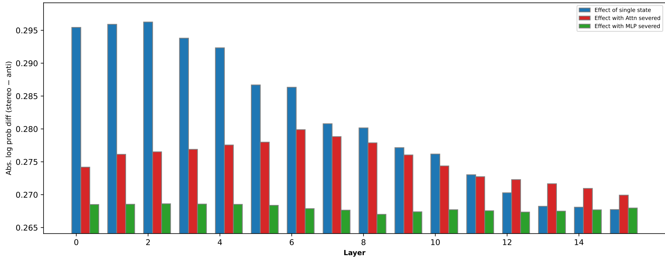
Race bias effect of states (OLMo-2-0425-1B [315B])
