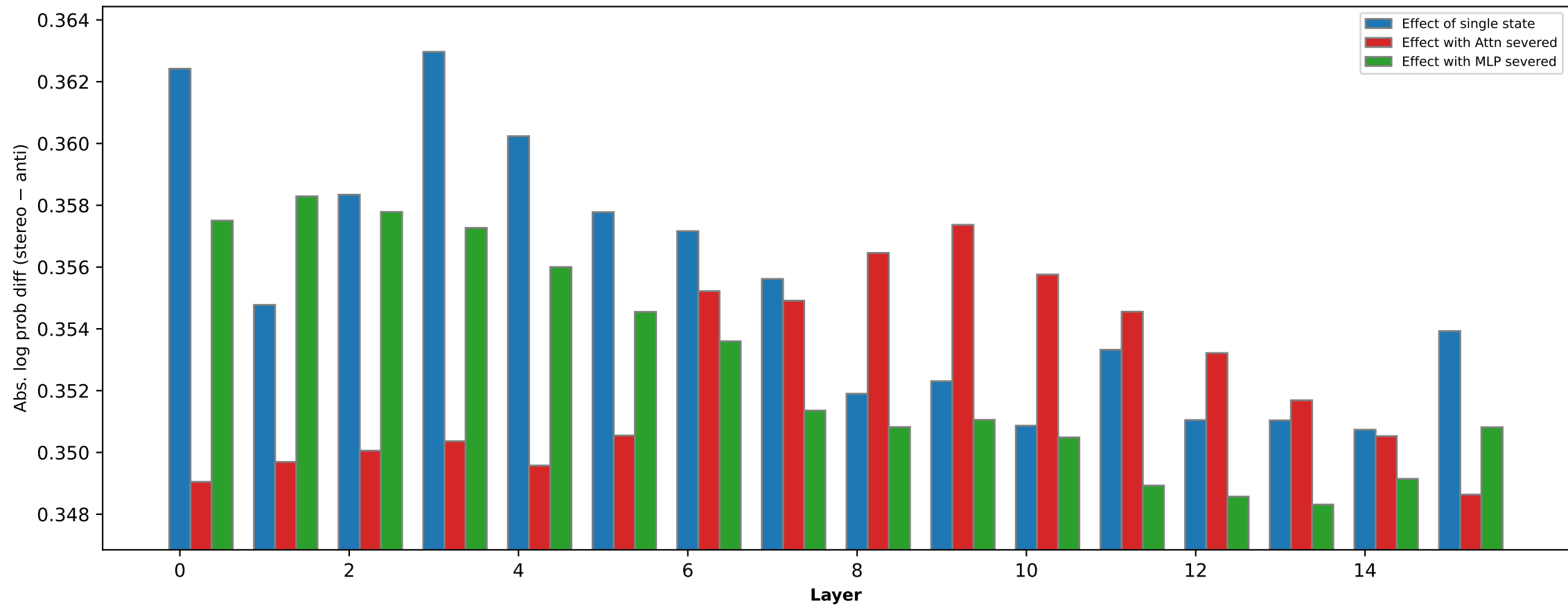
Religion bias effect of states (OLMo-2-0425-1B [315B])
