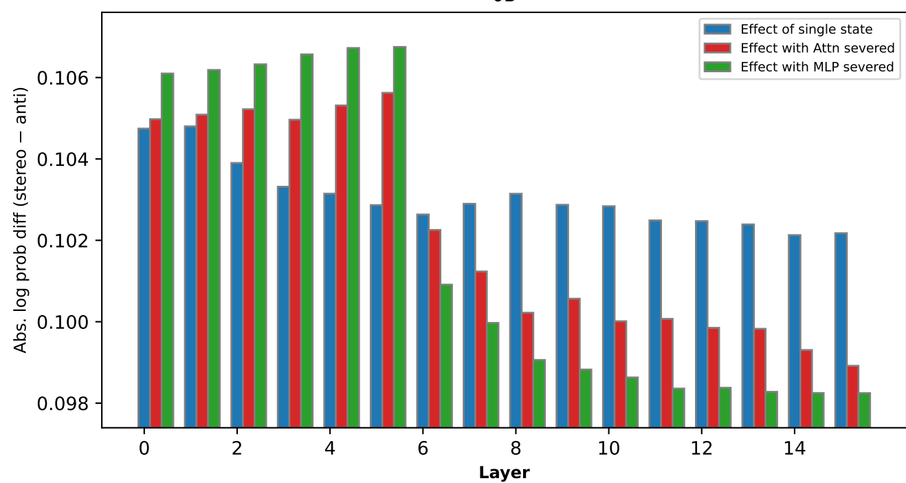
Gender bias effect of states — OLMo-2-0425-1B (all checkpoints)
