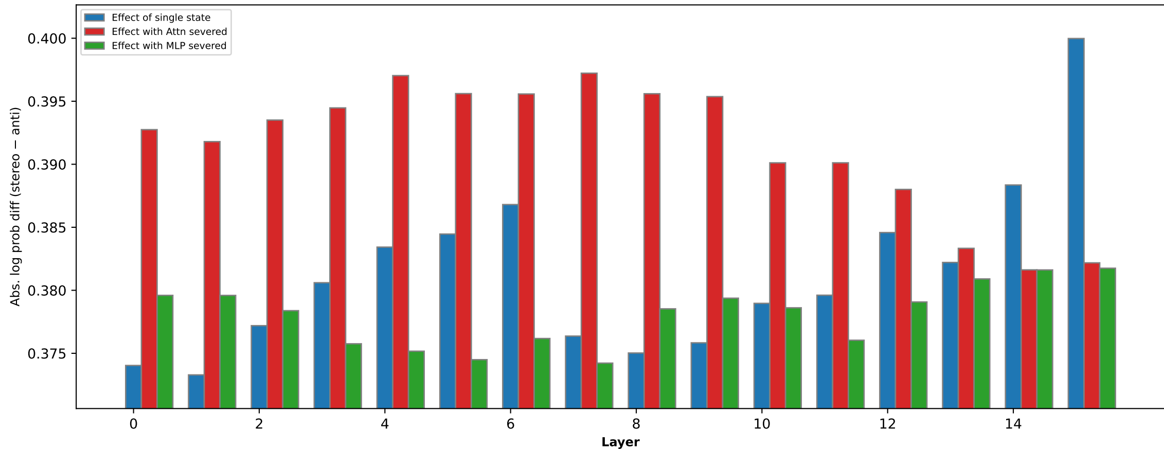
Religion bias effect of states (OLMo-2-0425-1B [main])
