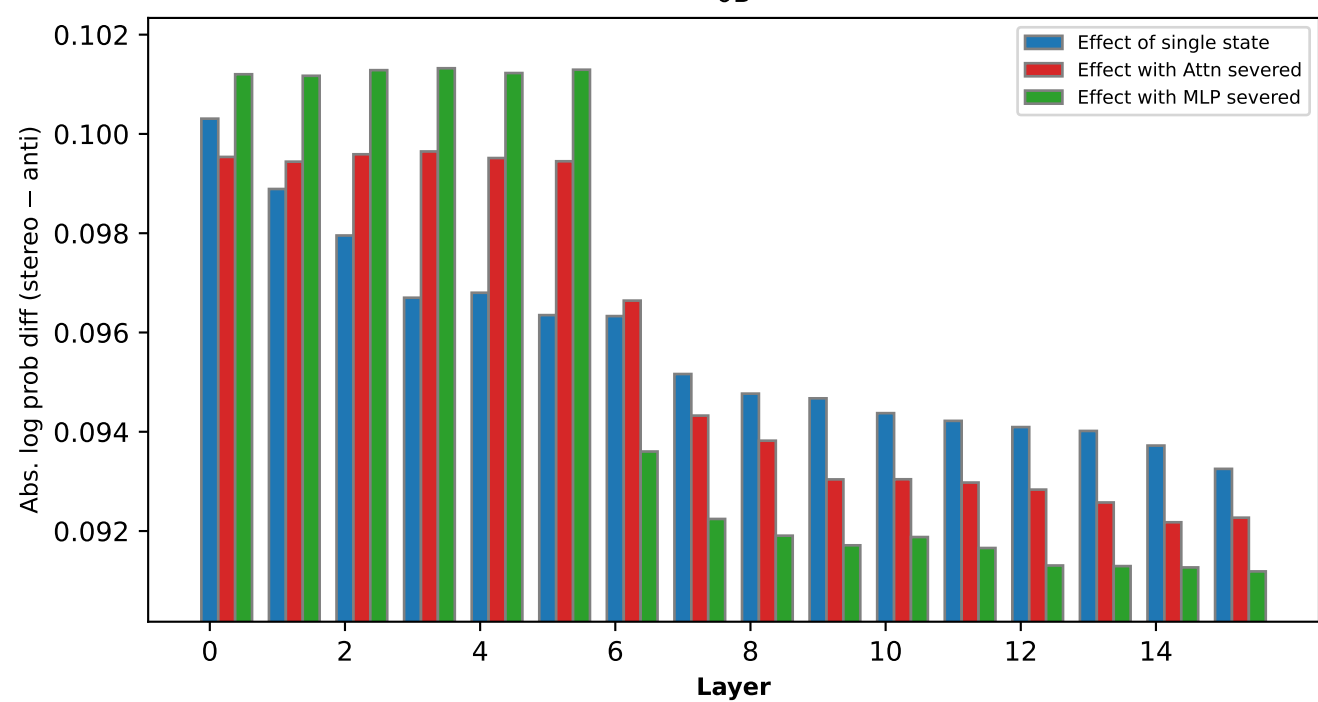
0B Profession bias effect of states — OLMo-2-0425-1B (all checkpoints)
