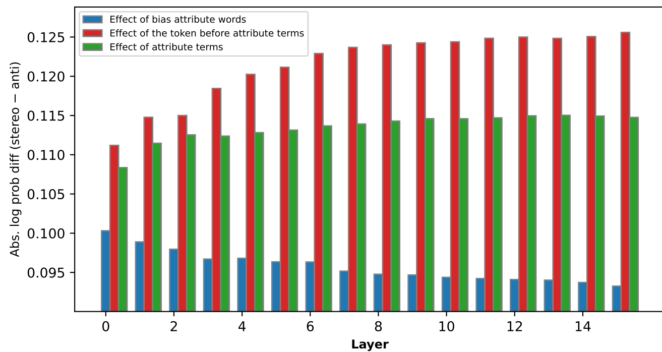
Profession bias effect of different words — OLMo-2-0425-1B (all checkpoints)
