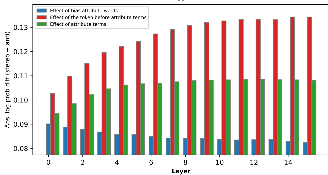
0B Race bias effect of different words — OLMo-2-0425-1B (all checkpoints)
