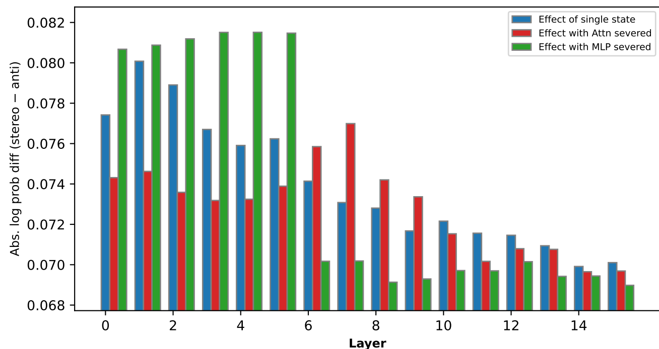
Religion bias effect of states — OLMo-2-0425-1B (all checkpoints)
