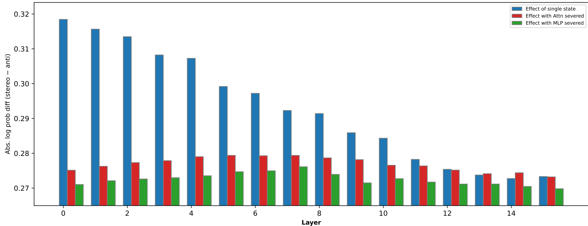
Profession bias effect of states (OLMo-2-0425-1B [s2-24B])
