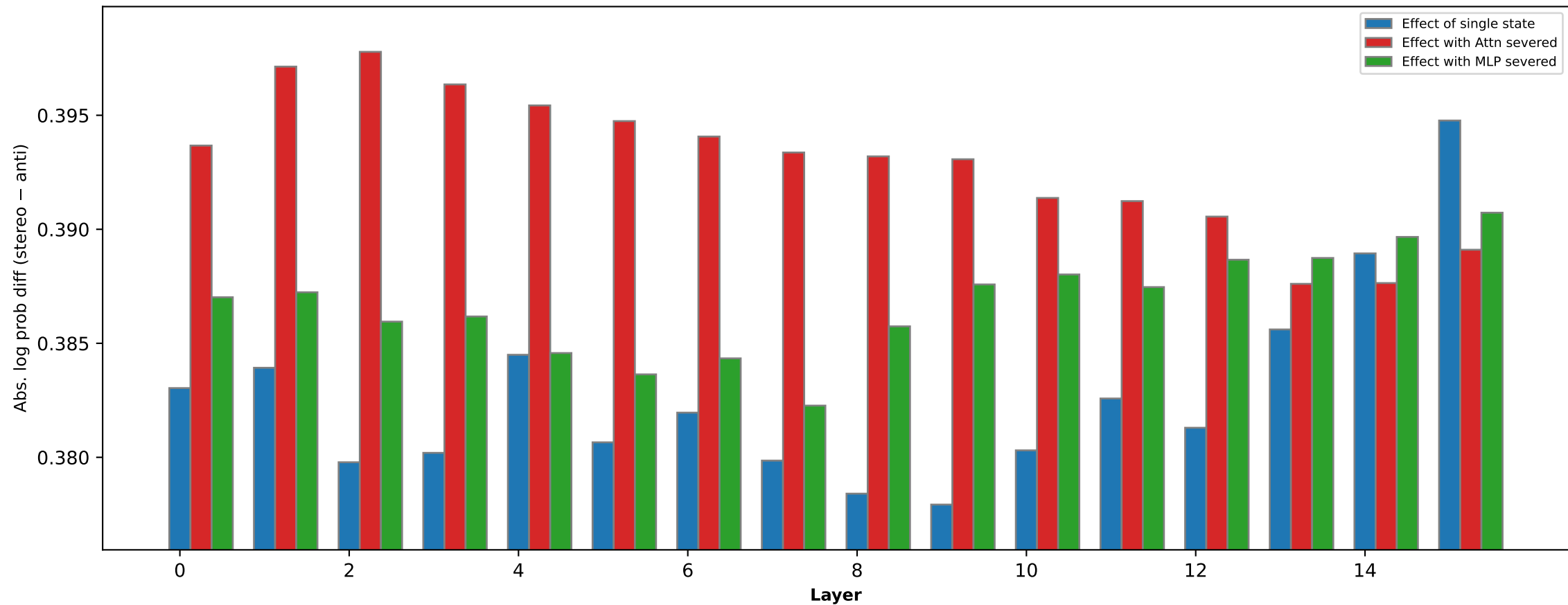
Religion bias effect of states (OLMo-2-0425-1B [s2-24B])
