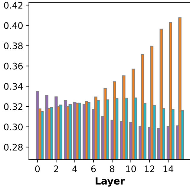
(h) Race bias effect of states (OLMo-2-0425-1B-Instruct)
