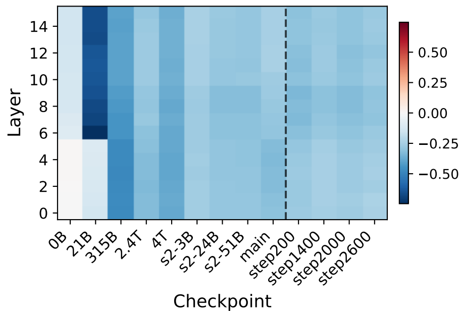
Effect with MLP severed
