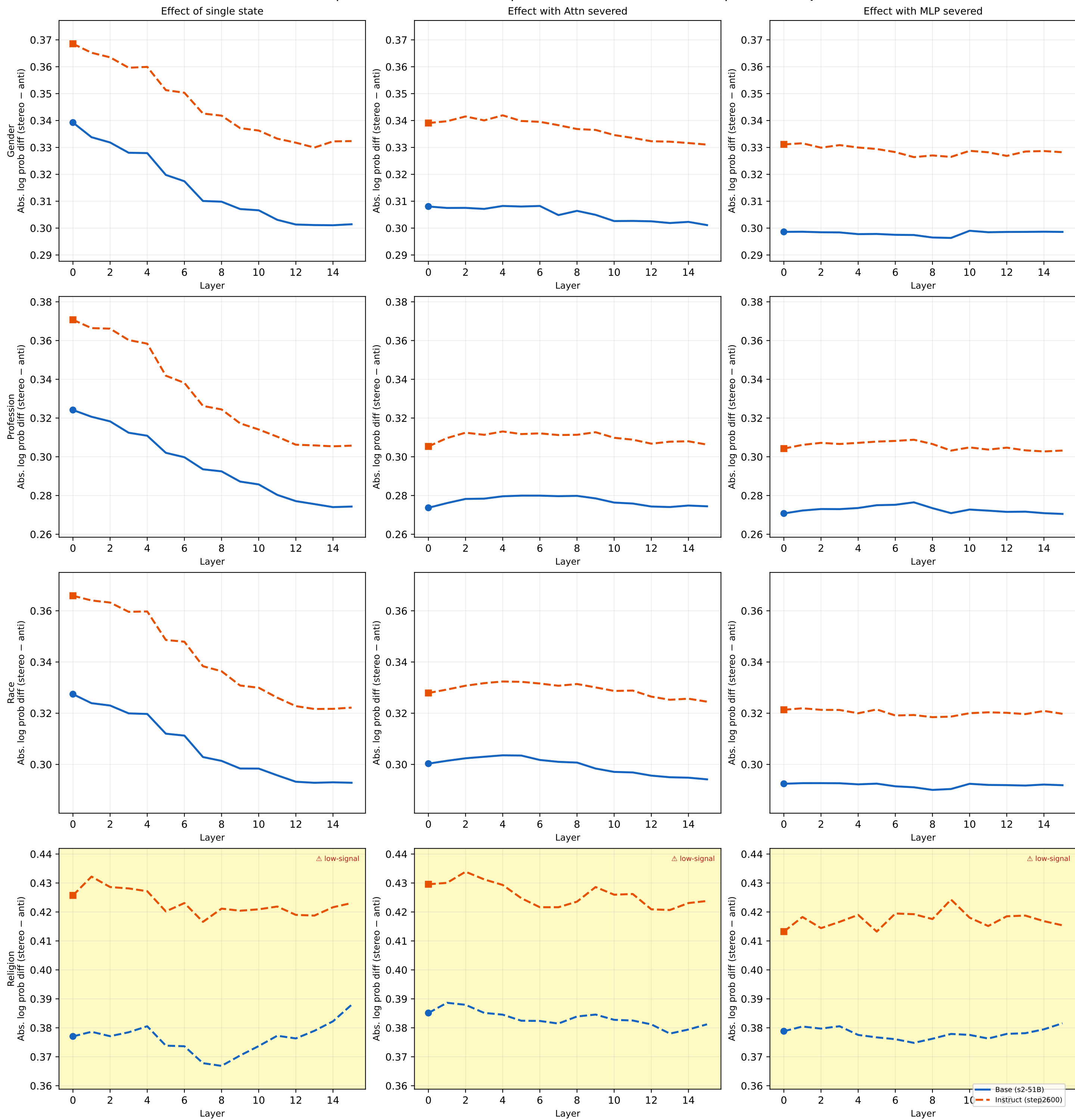
End of pretraining (s2-51B) vs end of post-training (step2600) — Abs. log prob diff Rows = domains | Cols = restore conditions | Solid = base, dashed = instruct | Y-axis fixed per row
