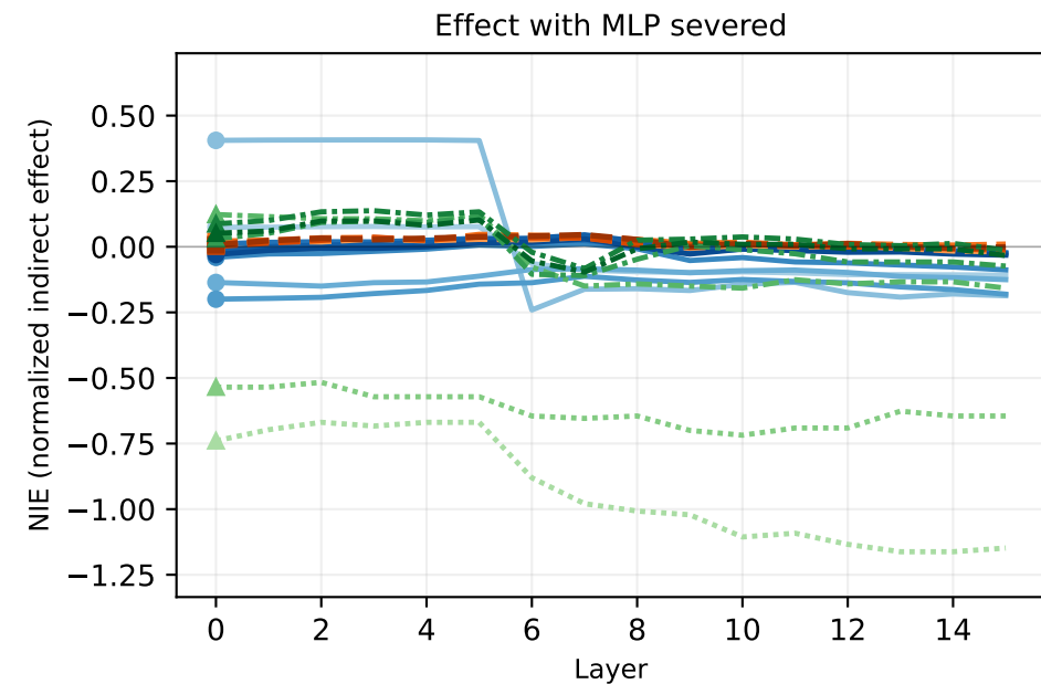
All models — Profession bias: layer profile comparison OLMo base (solid blue) · OLMo Instruct (dashed orange) · Pythia (dotted green). Y = NIE, shared across panels.
