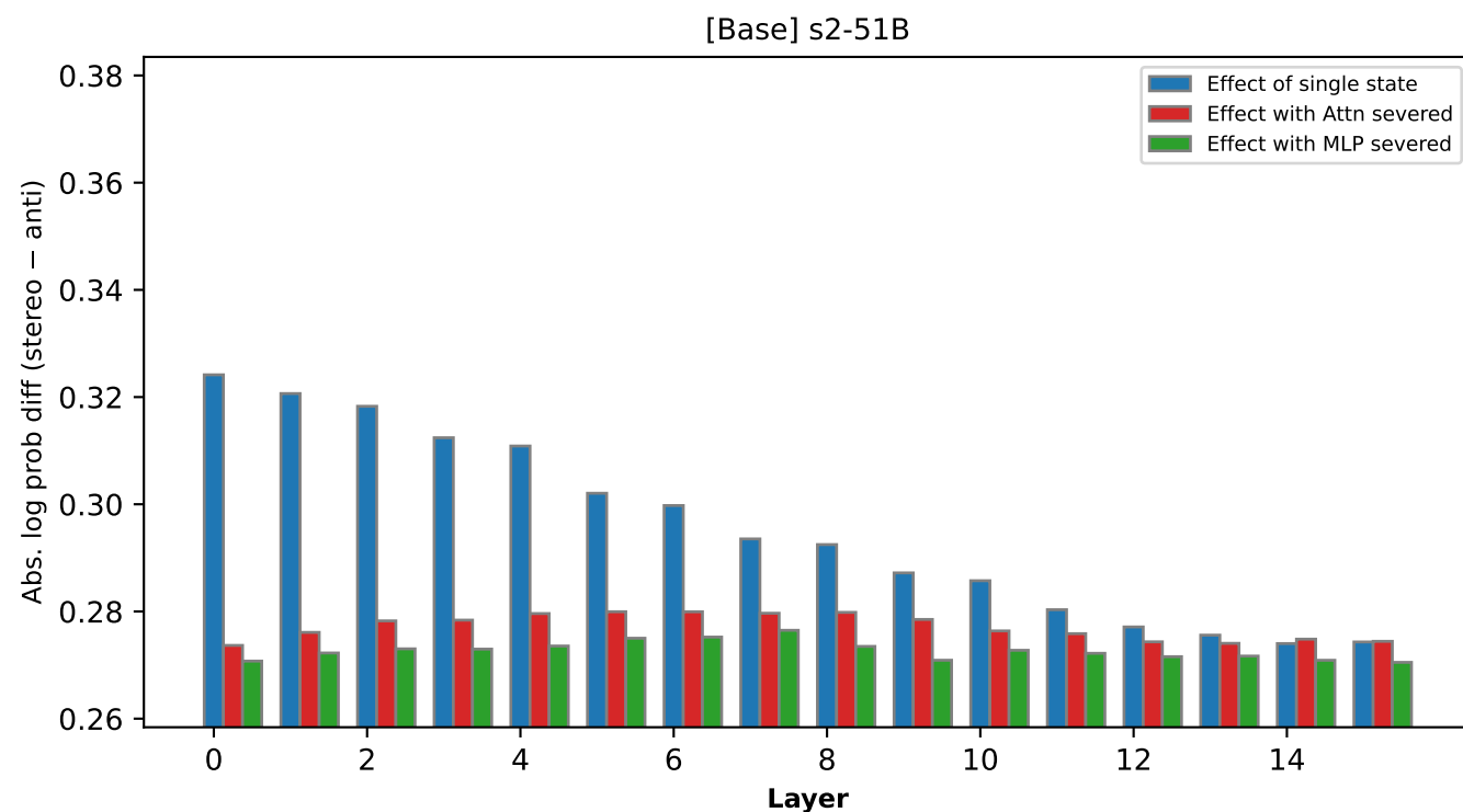
OLMo-2-0425-1B — Profession bias: Base vs Instruct Y-axis: Abs. log prob diff (stereo – anti). Fixed across all subplots.
