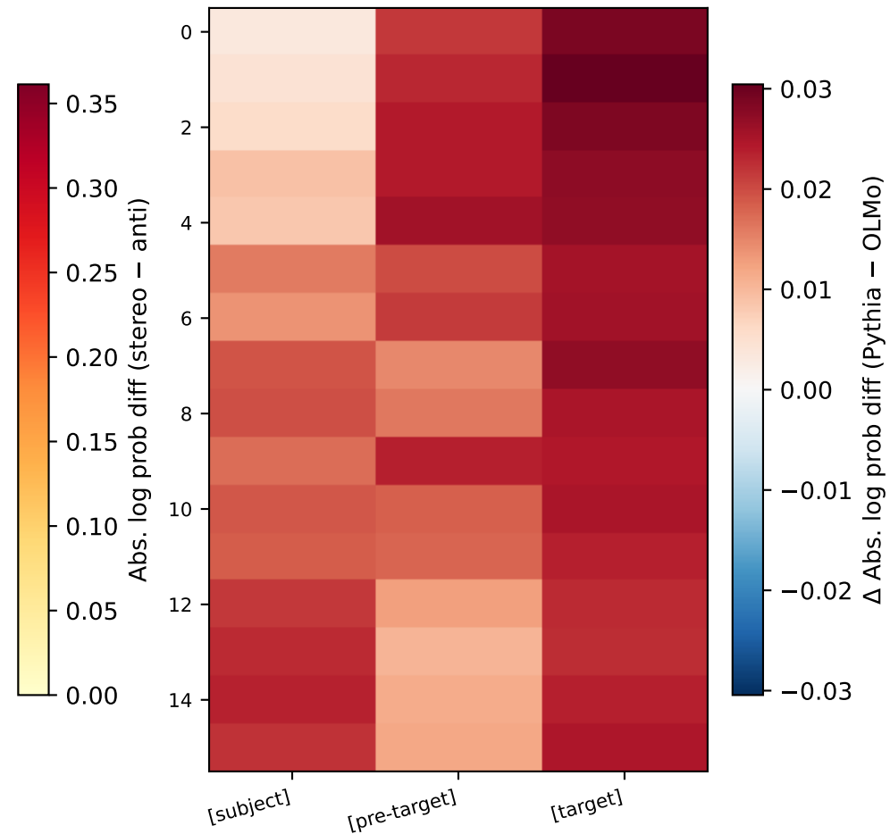
Profession — Pythia – OLMo
