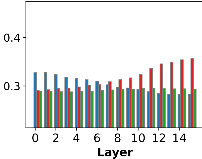
(a) OLMo-2-0425-1B (pre)
