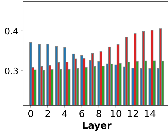
(b) OLMo-2-0425-1B-Instruct (post)
