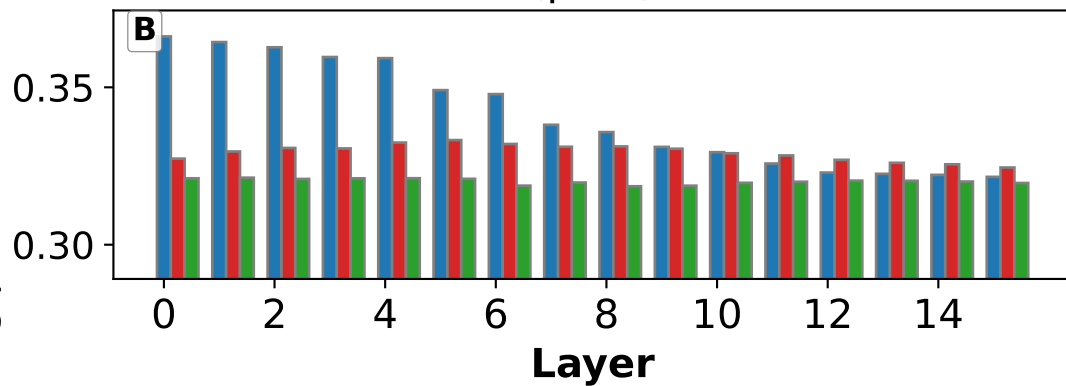
OLMo-2-0425-1B-Instruct (post)
