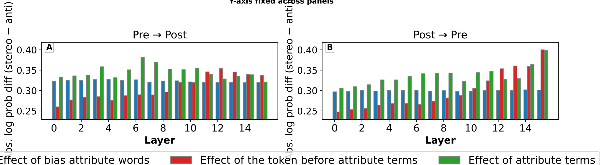
Race bias — cross-patch: Pre→Post vs Post→Pre (words) Y-axis fixed across panels
