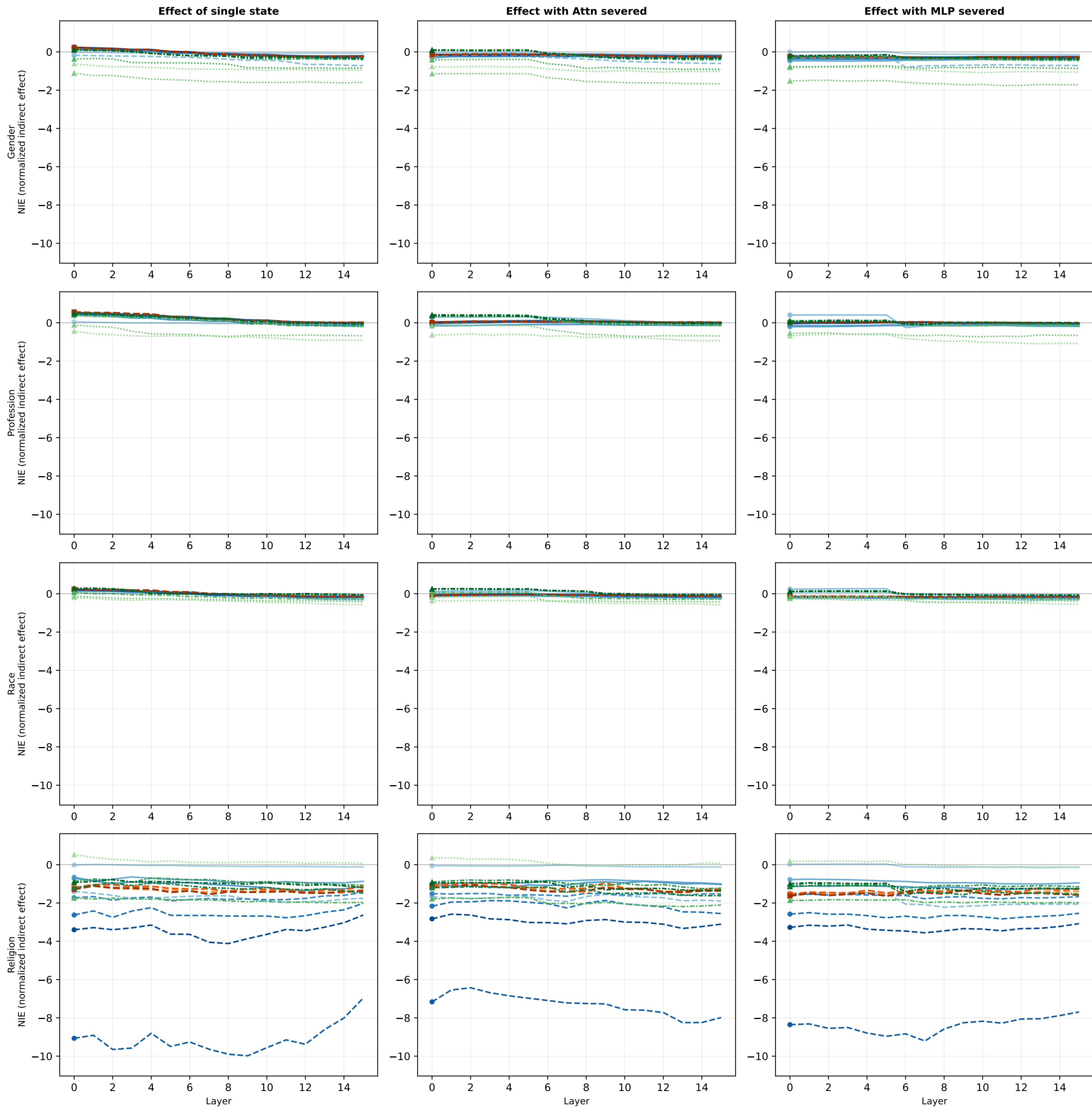
All domains × All models — layer profile comparison OLMo base (solid blue) · OLMo Instruct (dashed orange) · Pythia (dotted green). Y = NIE, fixed across all panels.
