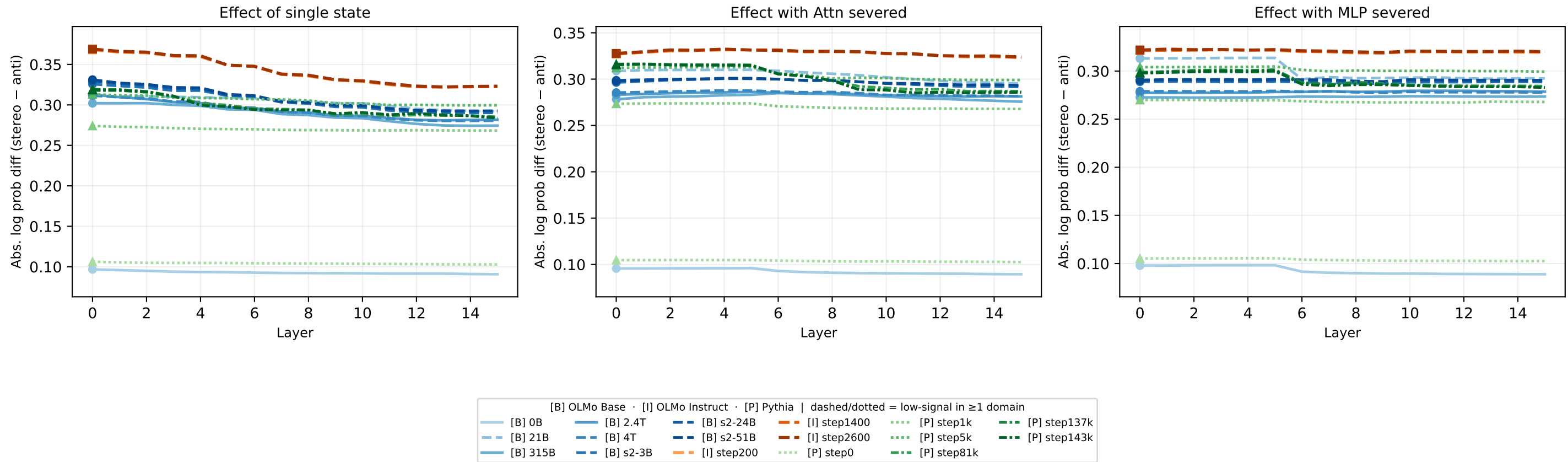
All models — Sentence-pair-weighted domain average: layer profile comparison Y = weighted mean abs log prob diff (weight = n_cases per domain). OLMo base (solid) · OLMo Instruct (dashed) · Pythia (dotted).
