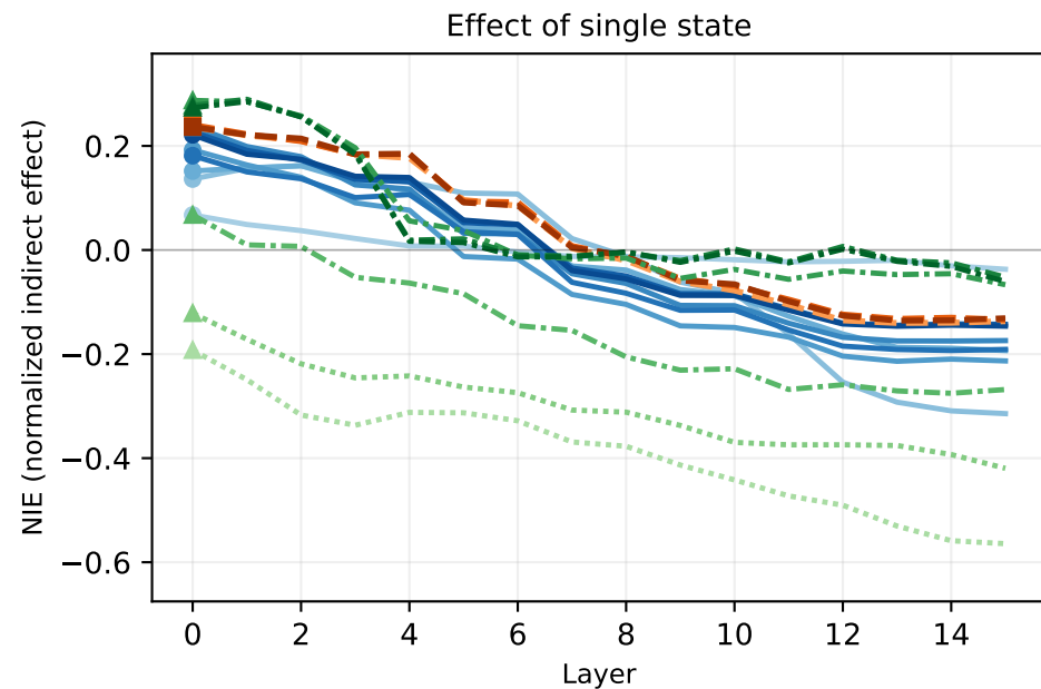
All models — Race bias: layer profile comparison OLMo base (solid blue) · OLMo Instruct (dashed orange) · Pythia (dotted green). Y = NIE, shared across panels.
