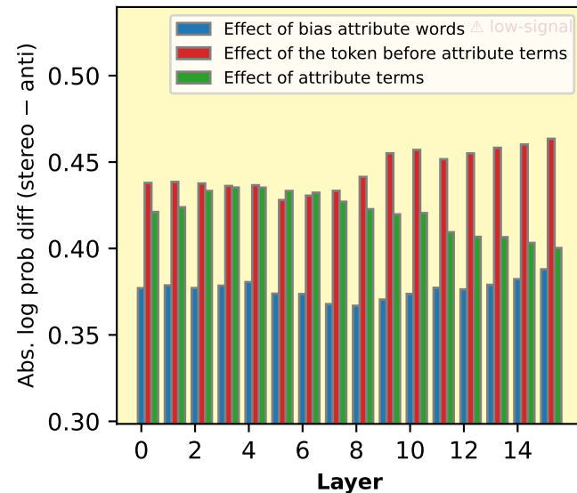
OLMo Stage 2 (s2-51B)
