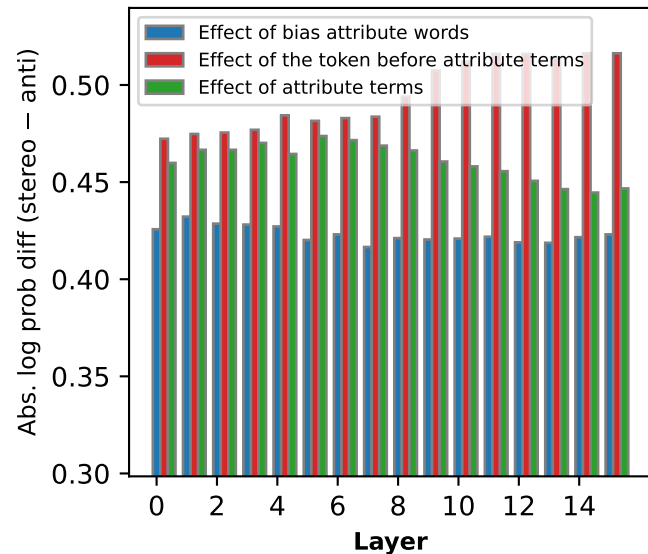
OLMo Instruct (step2600)
