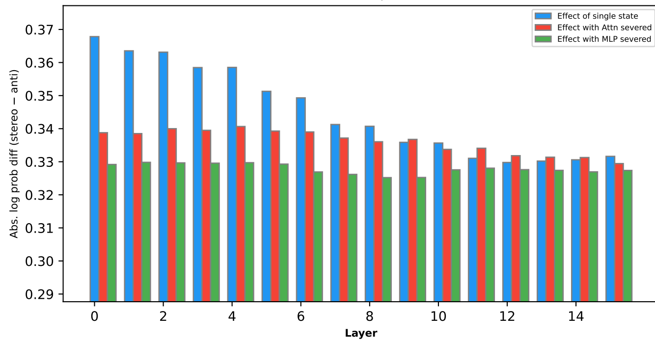
[Instruct] step1400
