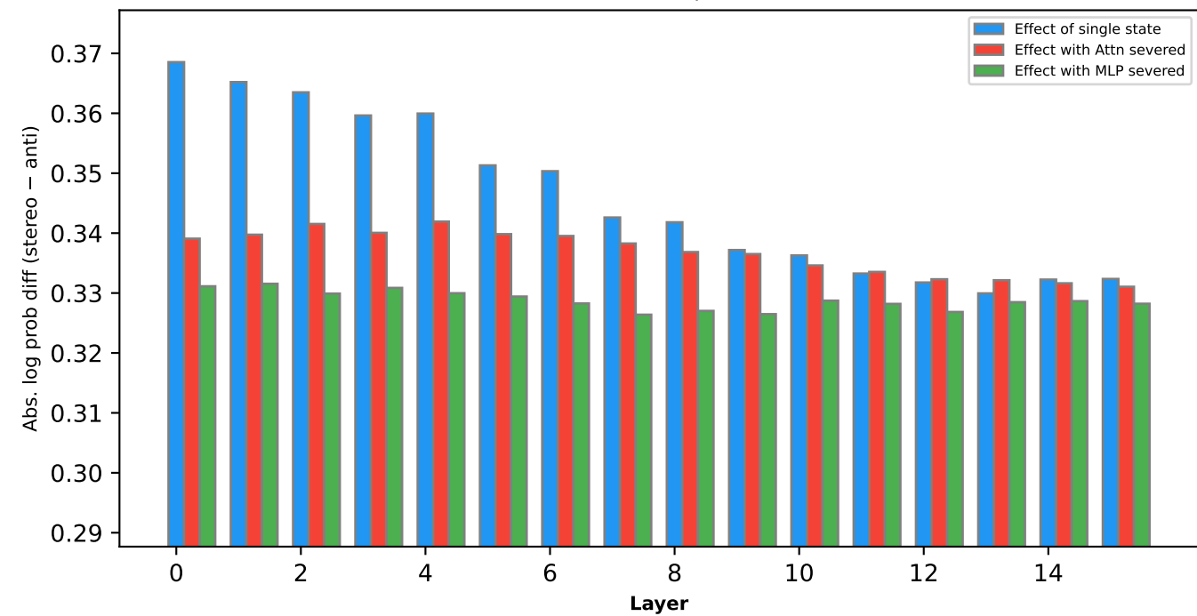
[Instruct] step2600
