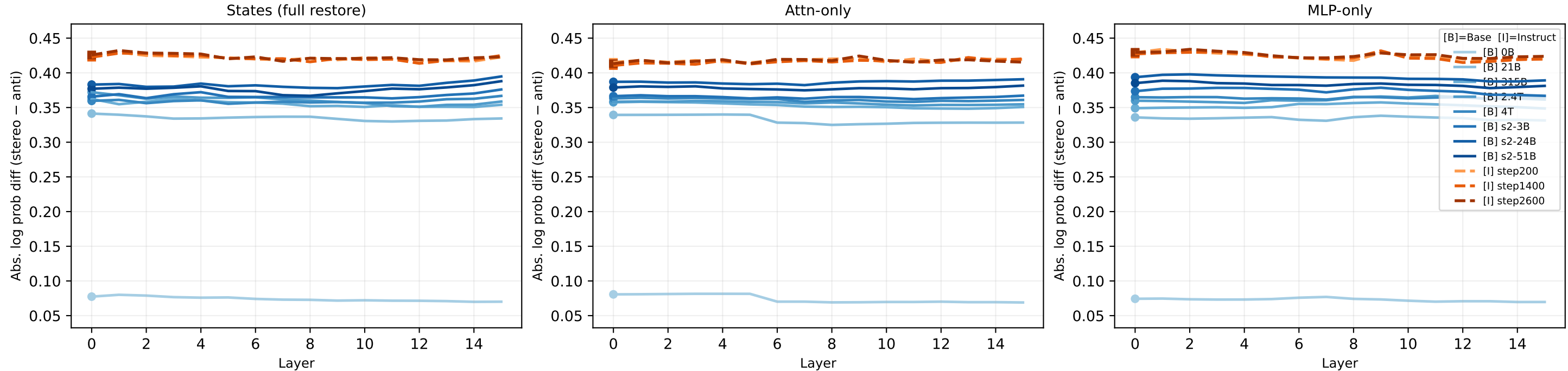
OLMo-2-0425-1B — Religion bias: Base (solid) vs Instruct (dashed) Each line = one checkpoint. X = layer, Y = abs. log prob diff (stereo – anti). Y-axis shared.
