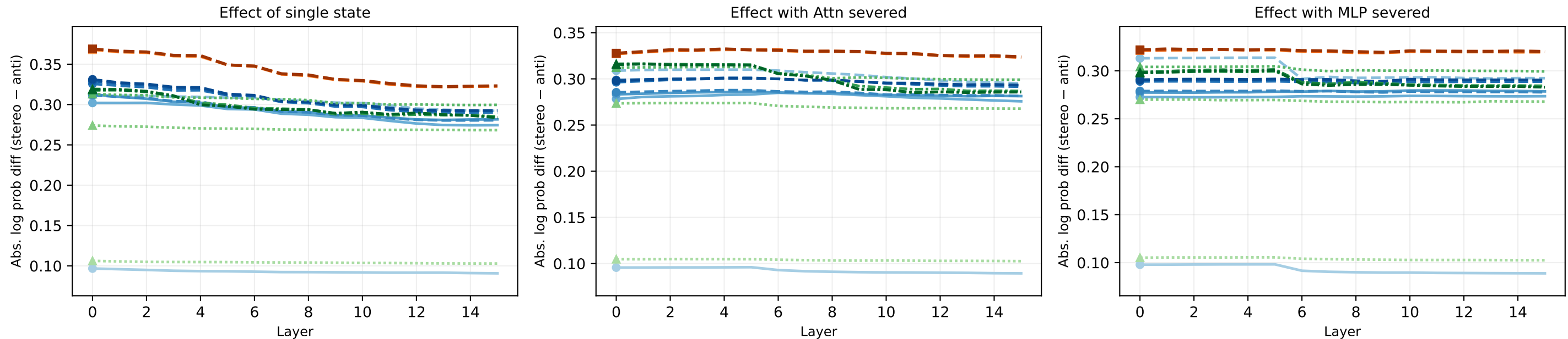
All models — Sentence-pair-weighted domain average: layer profile comparison Y = weighted mean abs log prob diff (weight = n_cases per domain). OLMo base (solid) · OLMo Instruct (dashed) · Pythia (dotted).
