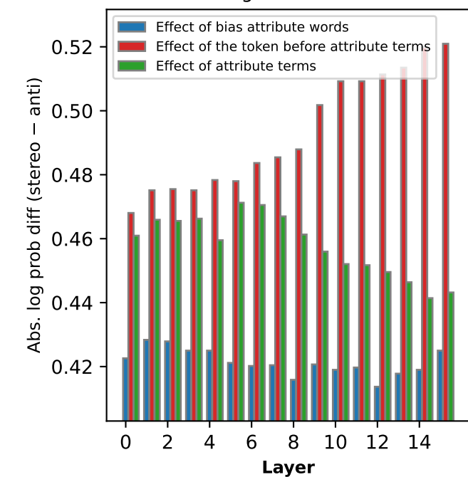
Religion — words
