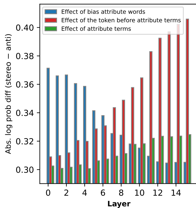
Profession — words
