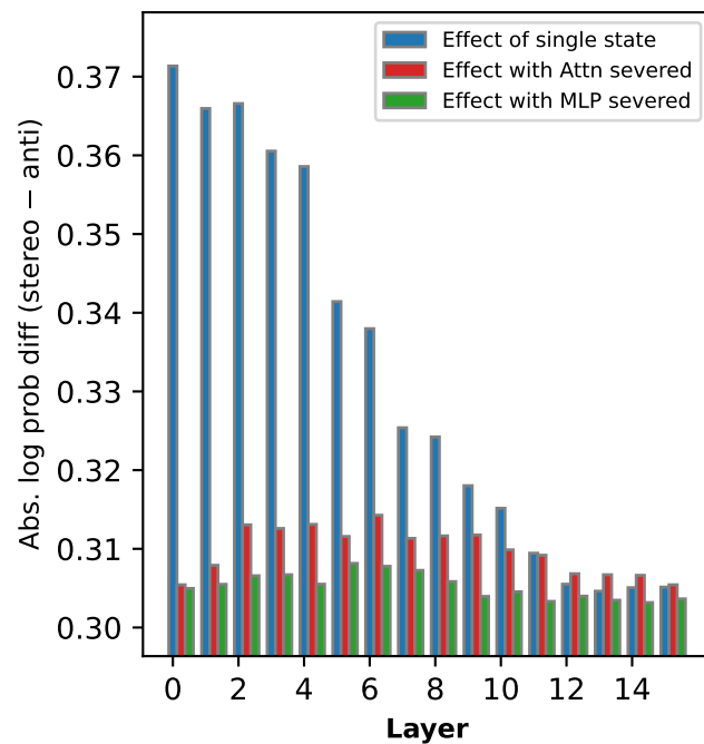
Profession — words
