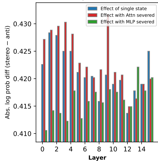
Religion — words
