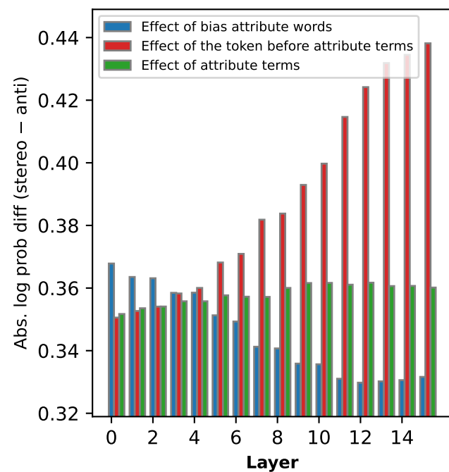
Gender — words
