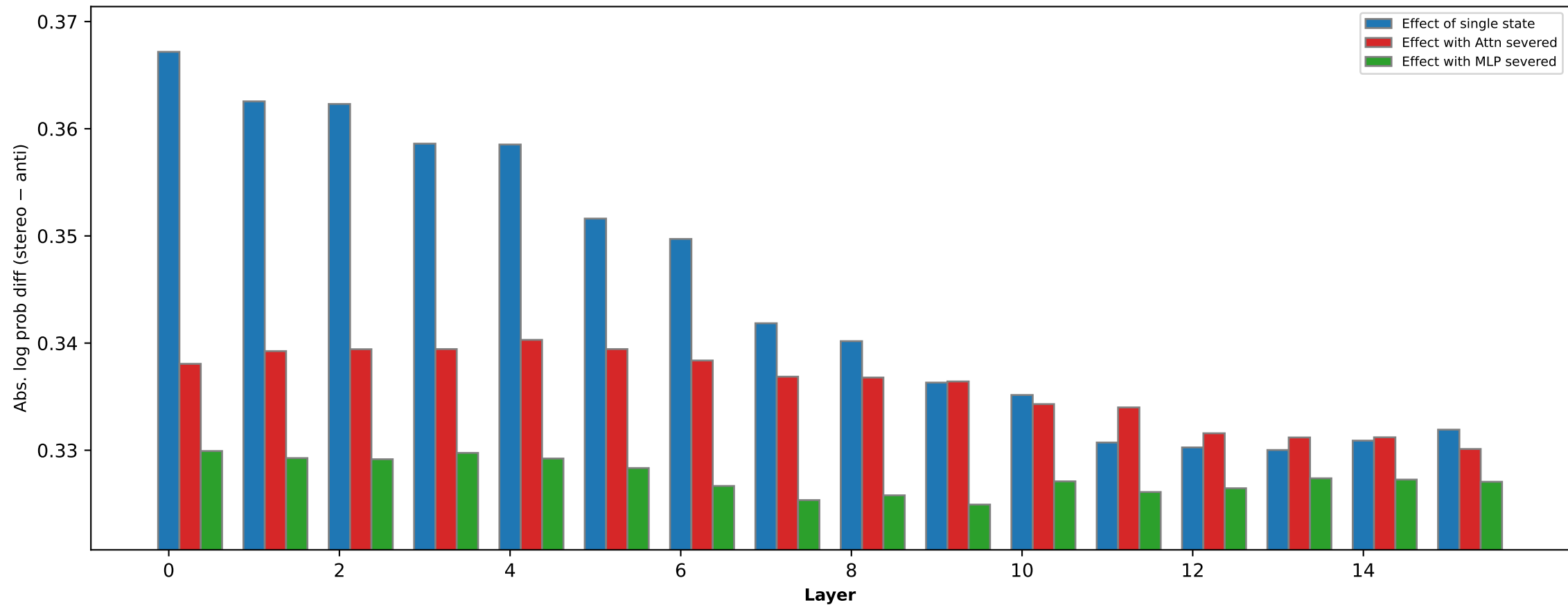
Gender bias effect of states (OLMo-2-0425-1B-Instruct [step200])
