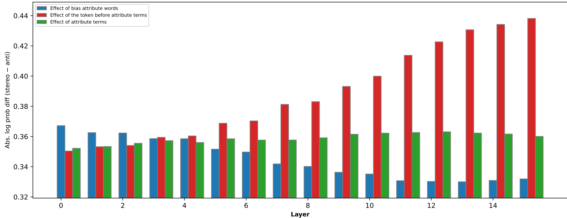
Gender bias effect of different words (OLMo-2-0425-1B-Instruct [step200])
