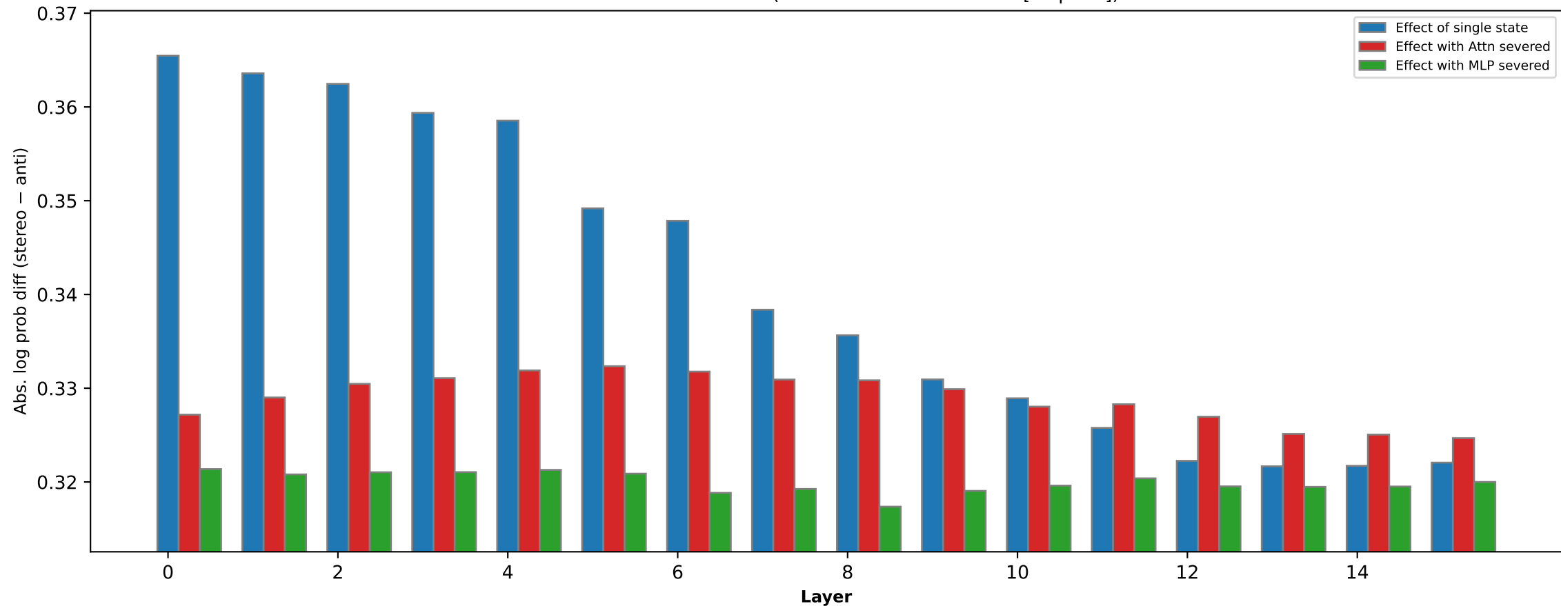
Race bias effect of states (OLMo-2-0425-1B-Instruct [step200])
