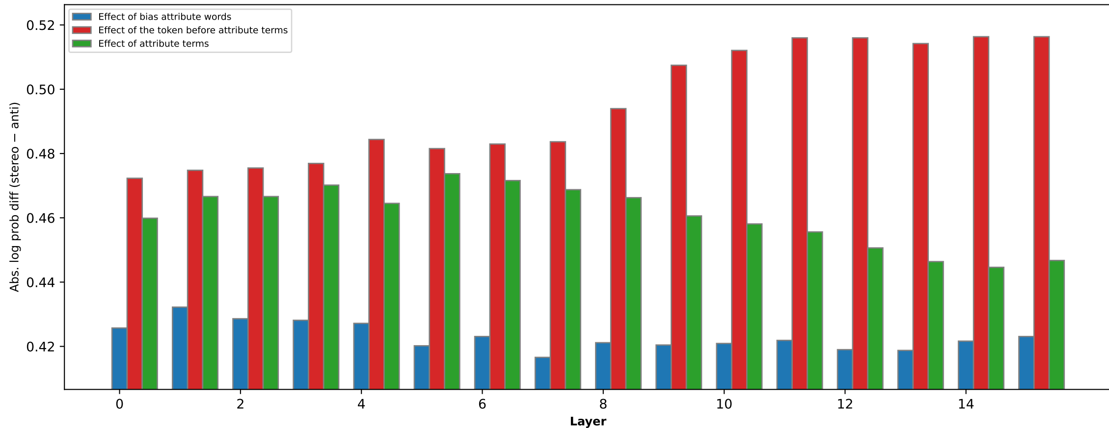
Religion bias effect of different words (OLMo-2-0425-1B-Instruct [step2600])
