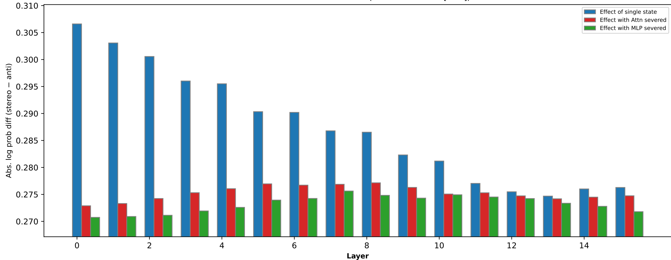
Profession bias effect of states (OLMo-2-0425-1B [2.4T])
