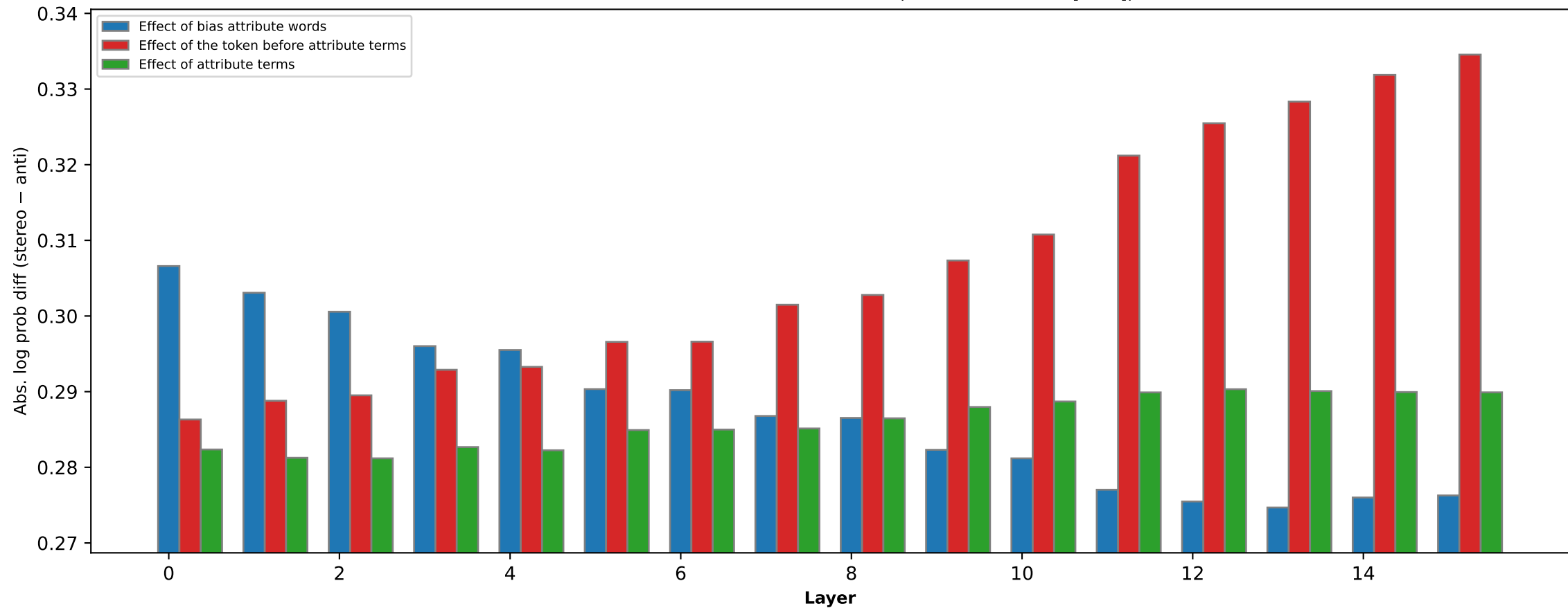
Profession bias effect of different words (OLMo-2-0425-1B [2.4T])
