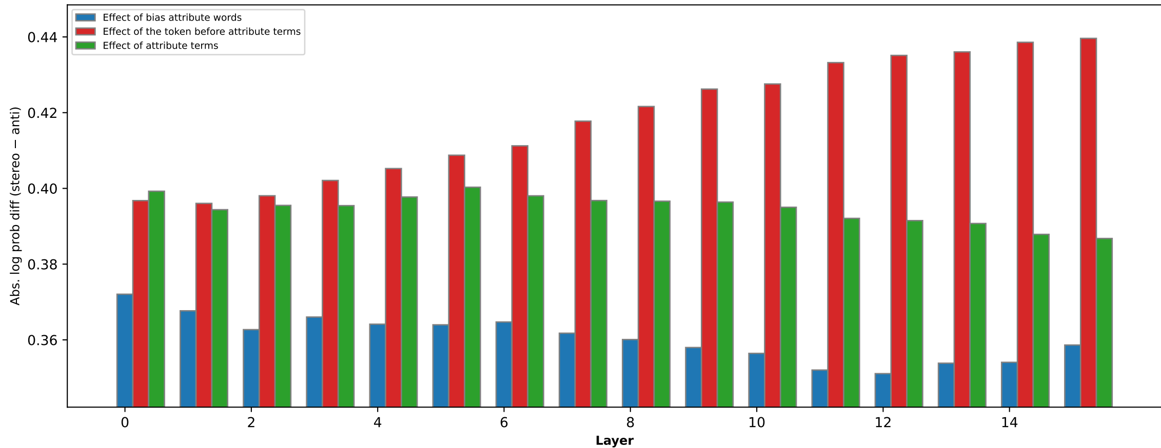
Religion bias effect of different words (OLMo-2-0425-1B [2.4T])
