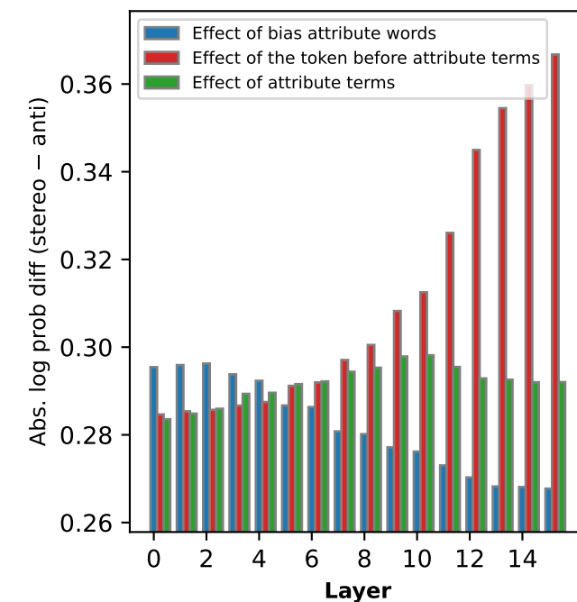
Race — words
