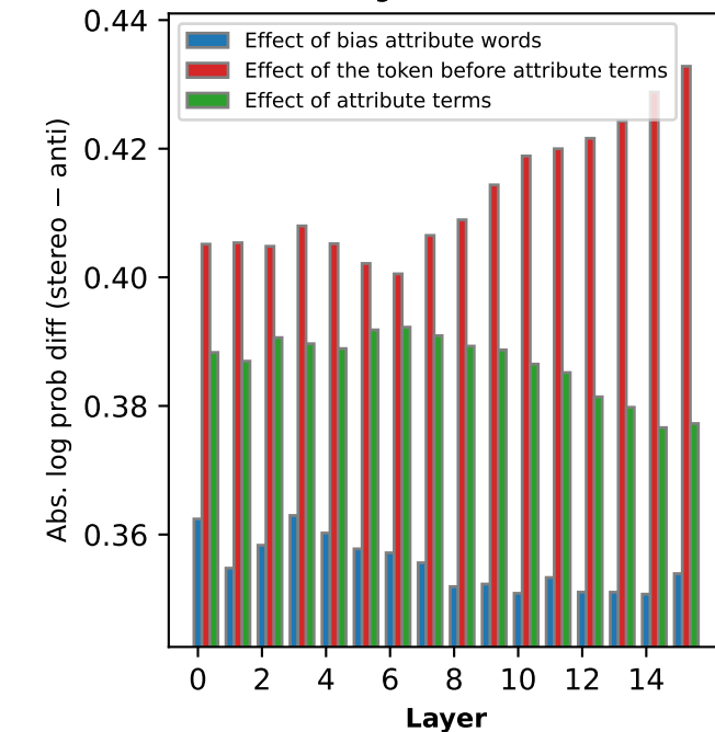
Religion — words
