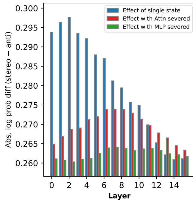
Profession — words
