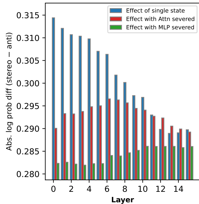
Gender — words
