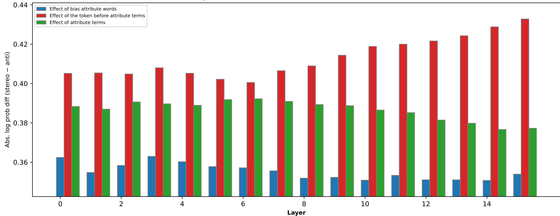
Religion bias effect of different words (OLMo-2-0425-1B [315B])
