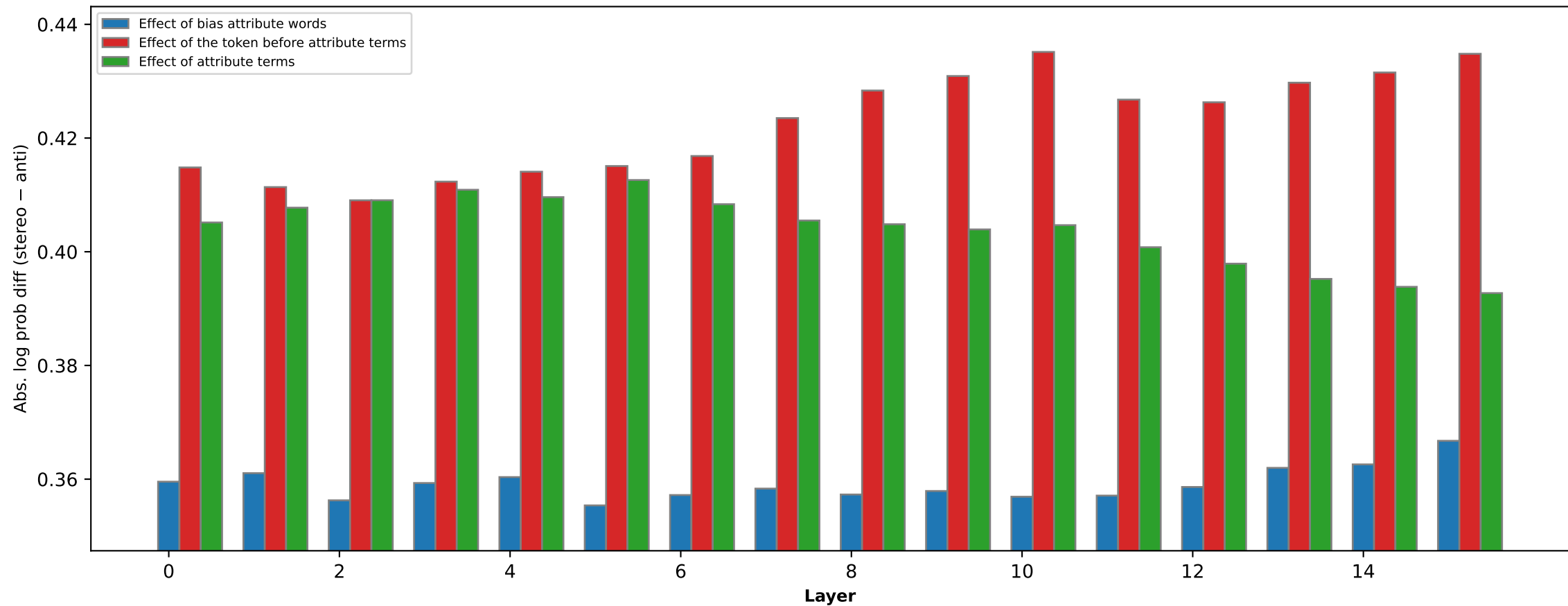
Religion bias effect of different words (OLMo-2-0425-1B [4T])
